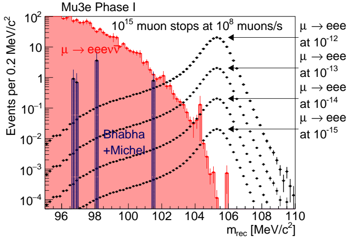
Figure 6: Expected invariant mass distribution of reconstructed \mu \rightarrow eee candidates. Background from the \mu \rightarrow eee\nu decays is shown in red and the dominant contribution to the accidental background in blue. The signal distribution (black points) is shown for different signal levels.
