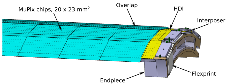
Figure 5: CAD drawing of an outer pixel tracker module: MuPix sensors with a thickness of 50\ \mu\text{m} are glued and spTAB-bonded on High Density Interconnects (HDI), thus forming ladders. The ladders are electrically readout via interposers and flexprints, and mechanically connected to end-pieces which also provide the helium gas cooling.
