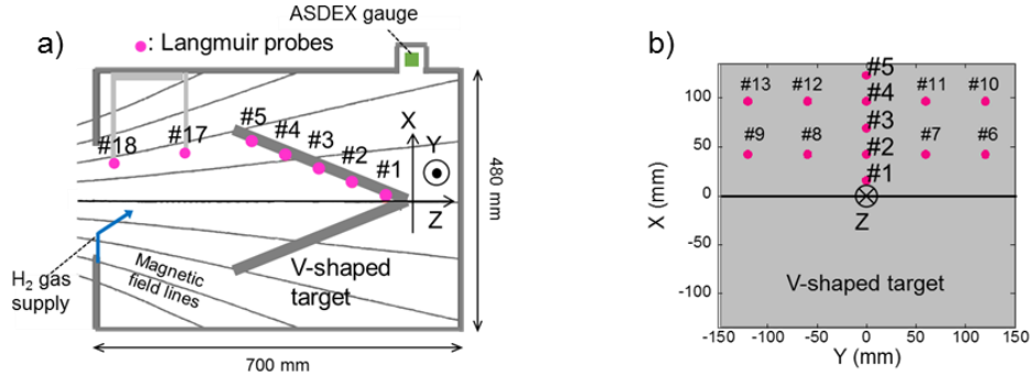
FIGURE 1. a) Schematic view of the D-module and b) array of Langmuir probes on the upper side of the V-shaped target. Probes are numbered as shown.
