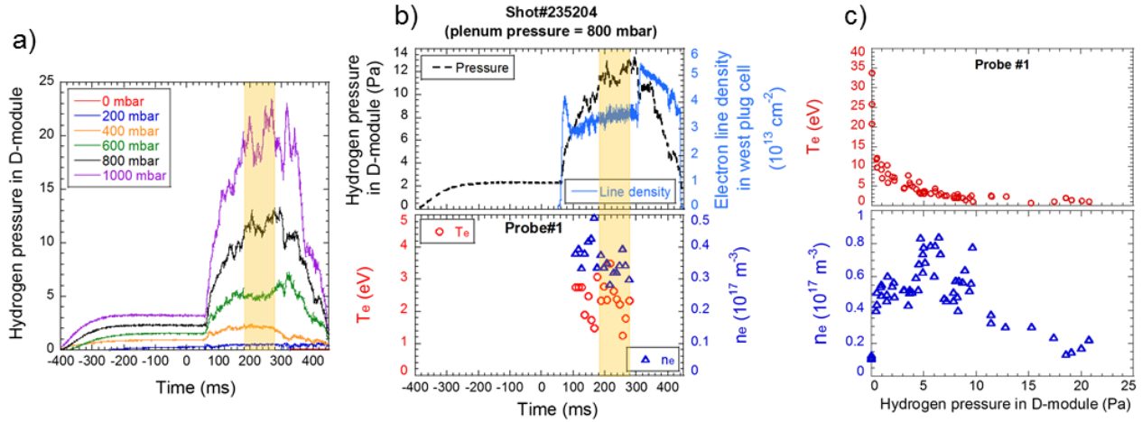
FIGURE 2. a) Time evolutions of hydrogen pressure measured by the ASDEX gauge in the D-module with respect to each initial plenum pressure (i.e. the pressure inside the reservoir tank behind the piezo valve) and b) hydrogen pressure and electron line density in the upstream west plug cell (top side) and electron temperature and density measured by Langmuir probe at the corner of the target (bottom side) as a function of time and c) electron temperature (top side) and density (bottom side) of the divertor simulation plasma measured by the corner probe in the hatched period in a) and b) as a function of hydrogen pressure in the D-module.
