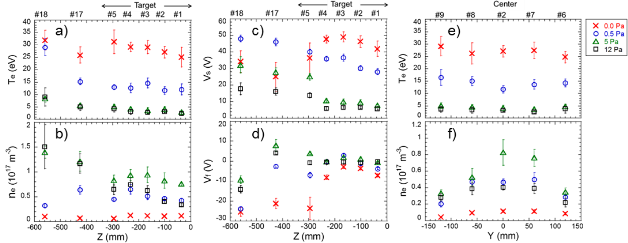
FIGURE 3. Distributions of a) electron temperature, b) electron density, c) space potential and d) floating potential measured by probes #1-5, #17 and #18, and distributions of e) electron temperature and f) electron density measured by probes #2 and #6-9. Those figures show comparison among the case without additional hydrogen gas supply (0.0 Pa) and the cases with the hydrogen pressures in the D-module of 0.5 Pa, 5 Pa, and 12 Pa.
