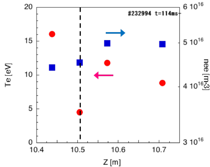
FIGURE 4. Electron temperature and electron density at several positions along Z-axis. The position indicated dotted line corresponds the place of the ISP. The other positions have Cardinal Langmuir probes.
