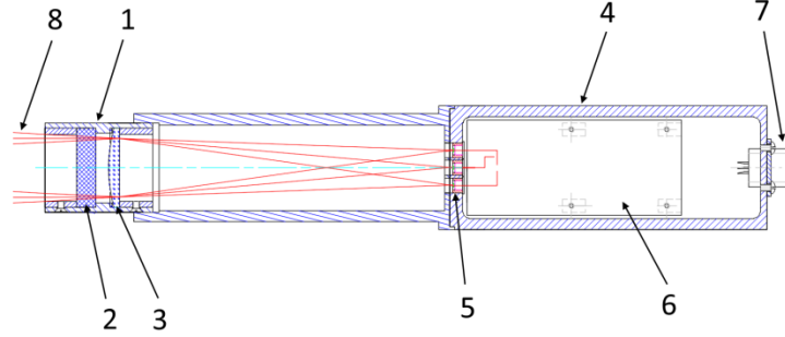
FIGURE 2. Three-channel measurement module: 1 – optical assembly, 2 – narrowband interference filter, 3 – plano-convex lens, 4 – electronics box, 5 – APDs, 6 – printed circuit board with amplifiers, 7 – power and signal connectors, 8 – input light rays.
