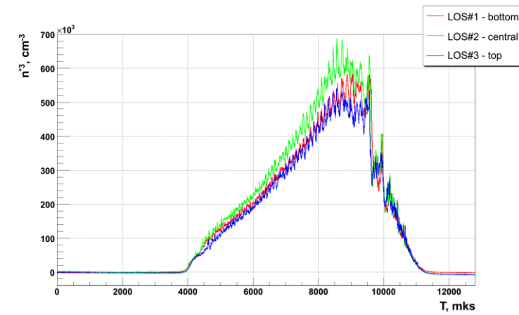
FIGURE 4. Signals obtained in shot #40123.
