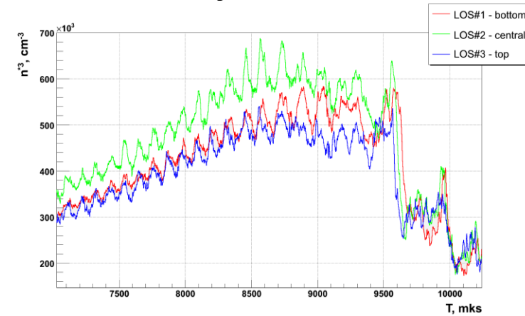
FIGURE 5. Signals obtained in shot #40123 (scaled).
