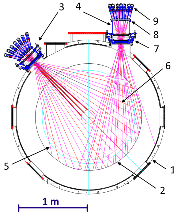
FIGURE 1. Layout of the optical 2D tomographic diagnostic: 1 – cross section of the vacuum vessel of the plasma installation, 2 – plasma boundary, 3 – “WIDA-diameter” bundle, 4 – “WIDA-radius” bundle, 5 – line of sight, 6 – area of best accuracy of tomographic reconstruction, 7 – two-axis angular aligning unit, 8 – measurement module holder with temperature stabilization, 9 – three-channel standard measurement module.
