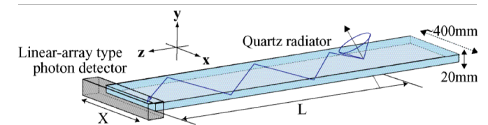
Early Belle II TOP design
