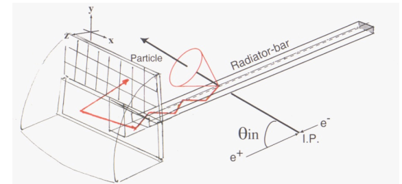
Early SuperB fDIRC design
