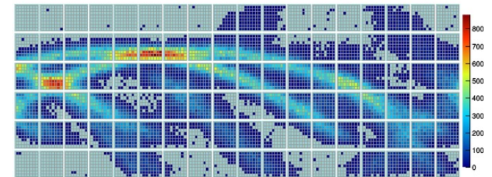
Geant4 hit pattern, 4GeV/c kaons
