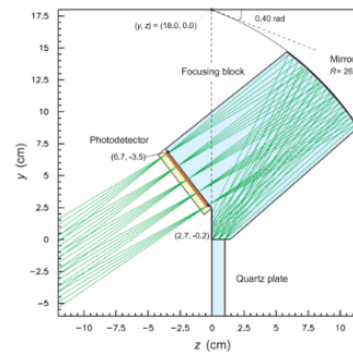
Photons from primary track
