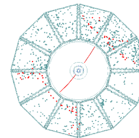
Typical event BaBar DIRC
