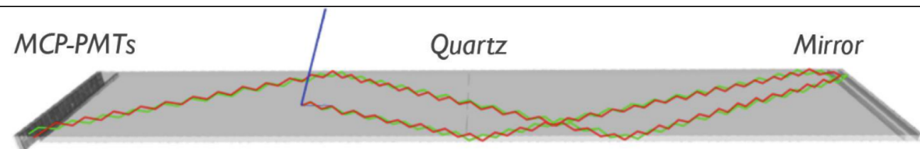
Example of Cherenkov-photon paths for 2 GeV/c \pi^+ and K^+ .
