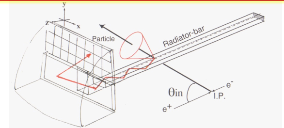
Early SuperB fDIRC design
