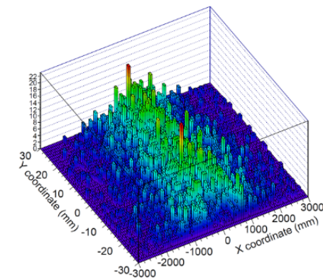
Photons from secondary tracks
