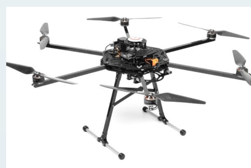
Examples of manufactured drones: the DS900 hexacopter for transporting loads up to 10 kg and a flight time of up to 40 minutes on one set of batteries (left); the DELTA h 1600 h drone with a load capacity of up to 7 kg and a flight time of up to 5 hours on a gasoline generator (right).
