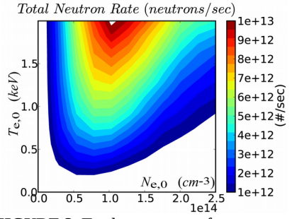
FIGURE 3. Total neutron rate from a GDT-like device, obtained as a function of central density and temperature from a set of a CQL3D simulations.
