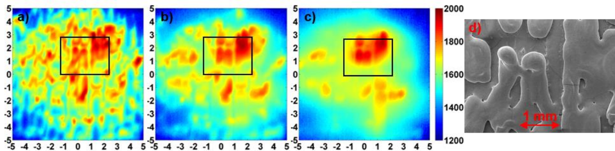
FIGURE 4. Temperature distribution after electron beam termination in different times: a) 350 \mu s, b) 1850 \mu s, c) 7850 \mu s. d) SEM picture of the area marked with black rectangular on previous images.
