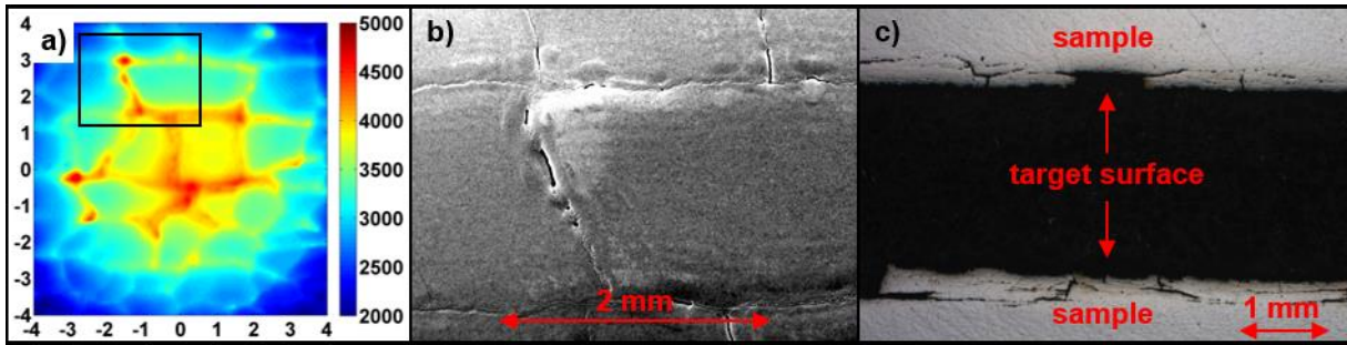
FIGURE 2. a) picture of temperature distribution on the surface 20 \mu s after beam impact; b) SEM image of the area marked with black rectangular on (a); c) transverse microsection of the sample
